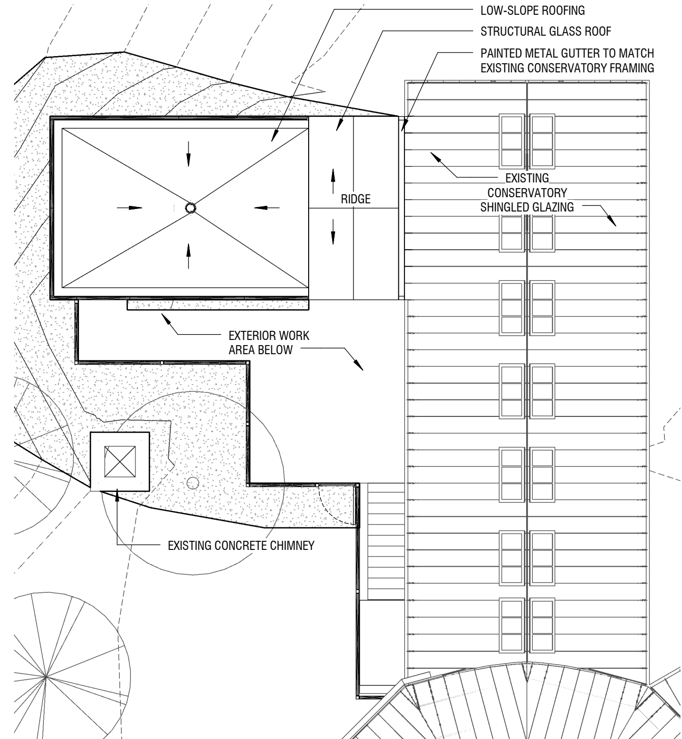
2 ROOF PLAN 1/8" = 1'-0"
