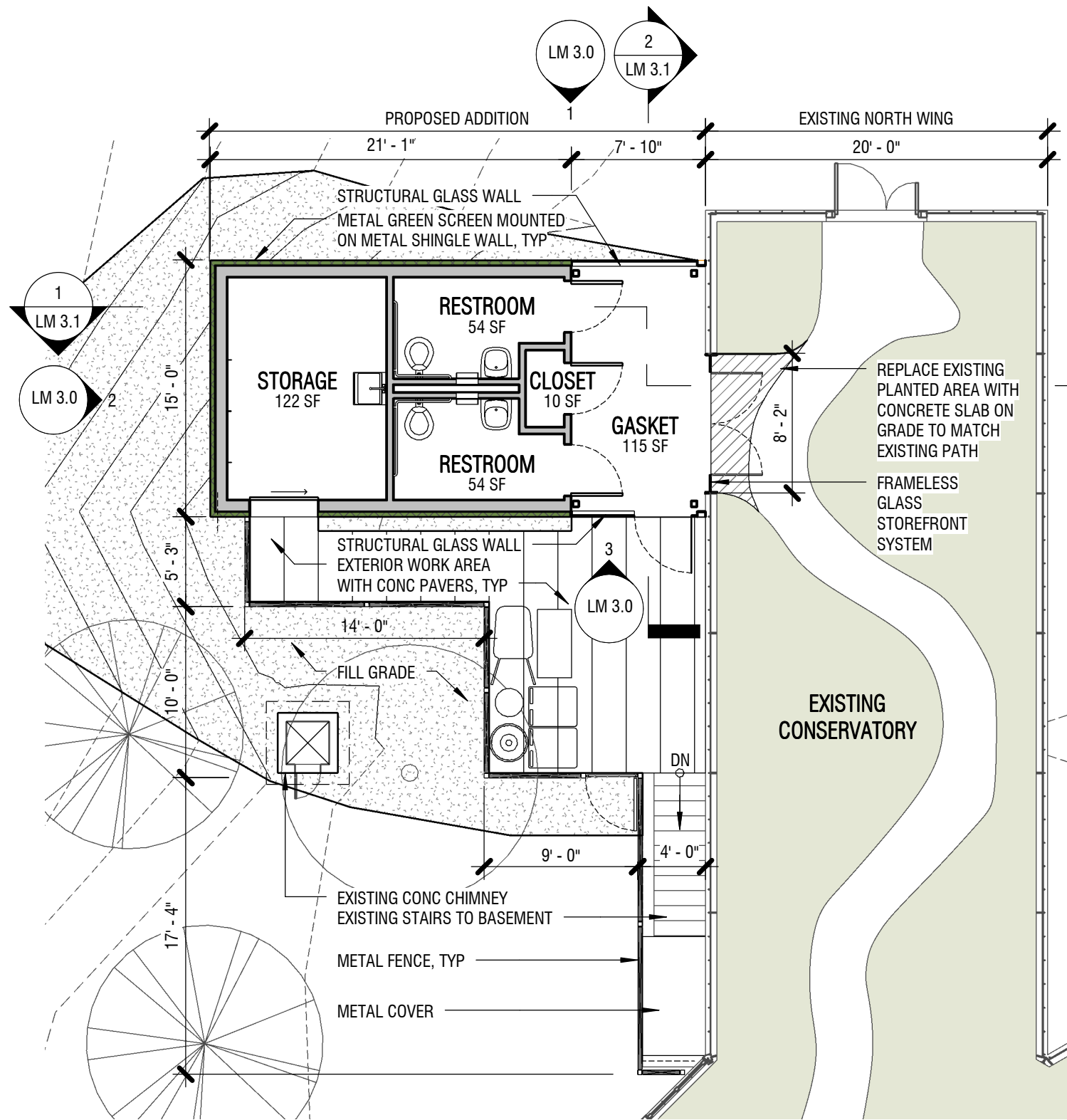
1 FLOOR PLAN 1/8" = 1'-0"
